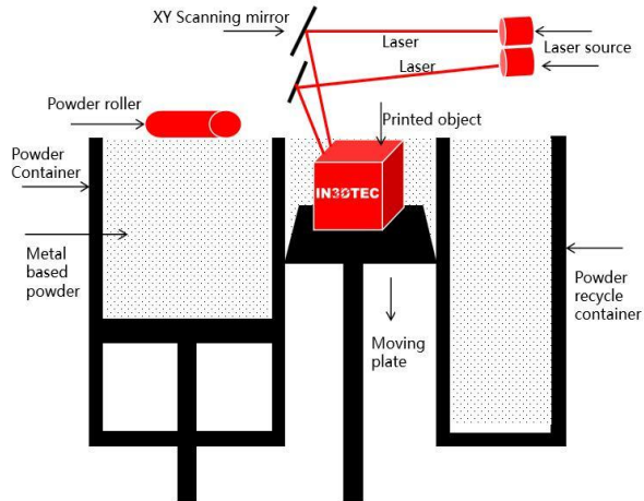
Laser Sintering, Laser Melting
