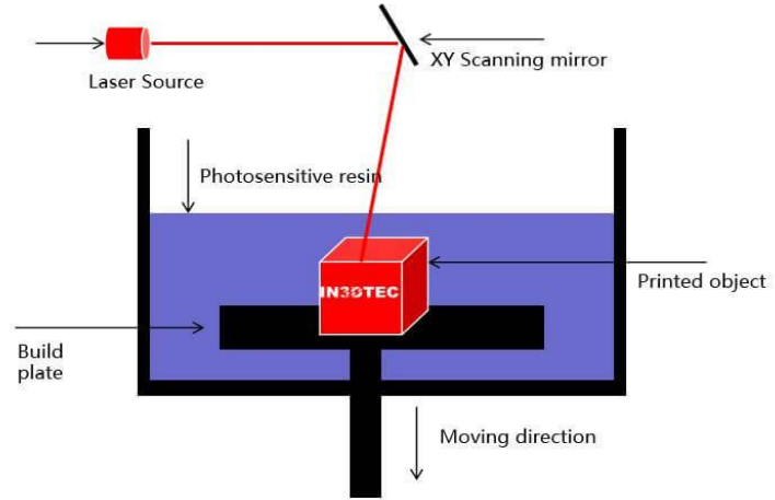
Stereolithography
