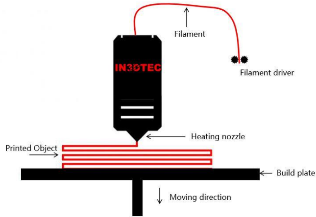
Fused Deposition Modeling
